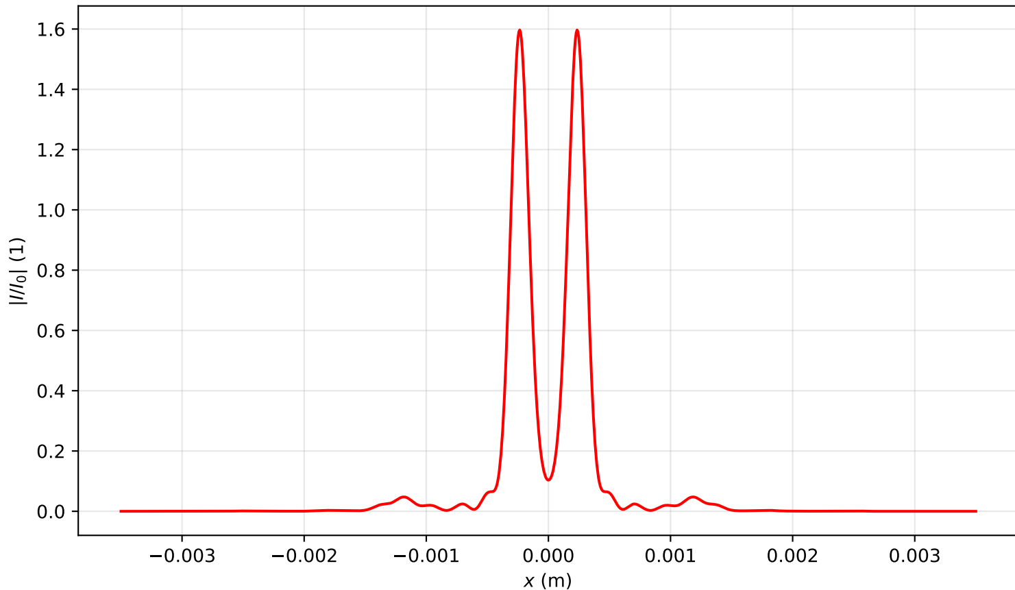
Intensity profile I(x, y = 0, z = 1.672)/I_0 , P_{in}=3.5P_{cr} , artificial time
